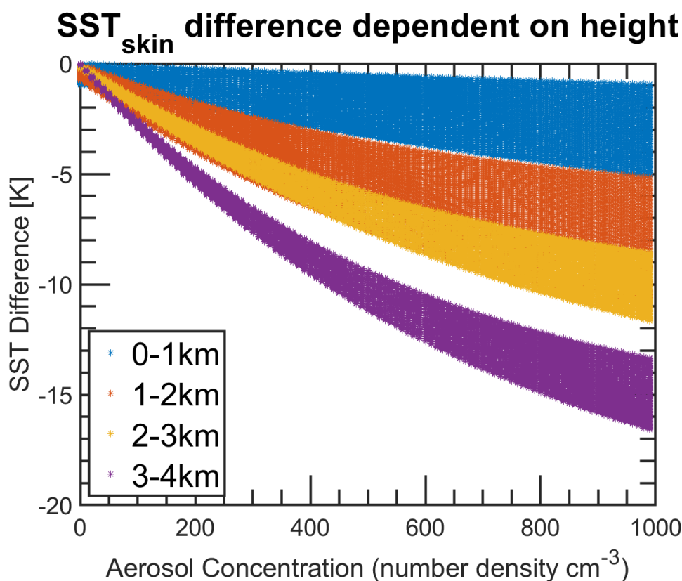
Figure 2. RTTOV simulation results showing the impact on the SST_{skin} retrieval of the altitude of the aerosol layer. Different colours indicate different altitudes of the dust layer. As the aerosol height is increased, the SST difference becomes more negative, except for very small concentrations.
