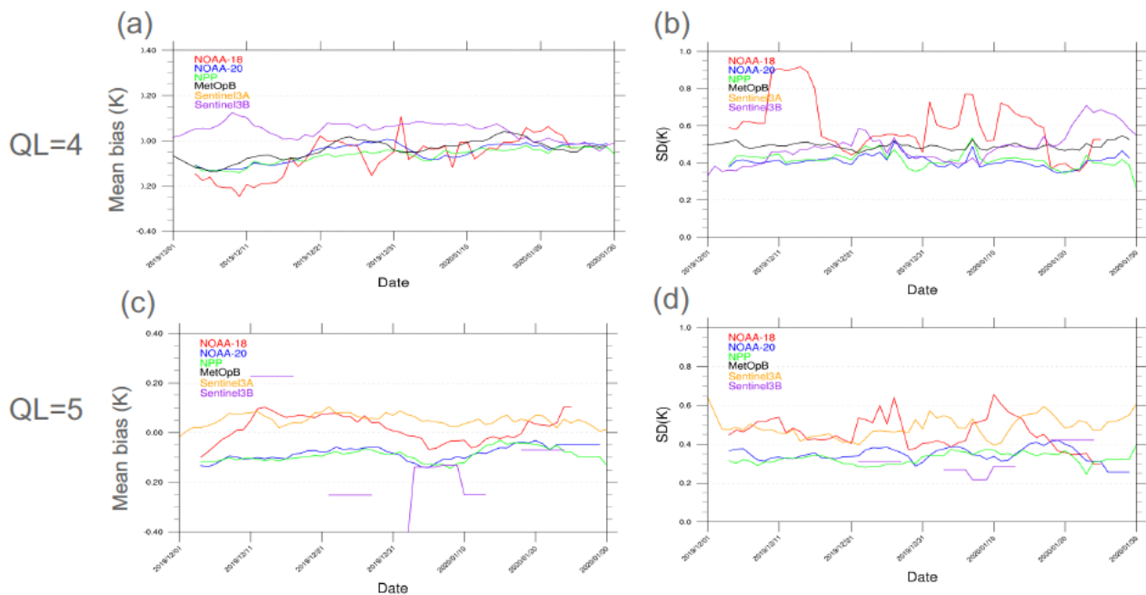
Figure 2: L3C-01day, night only, weekly statistics, 1 Dec 2019 - 31 Jan 2020, mean bias for (a) quality level 4 and (c) quality level 5, and standard deviation for (b) quality level 4 and (d) quality level 5, when compared with Drifting and tropical Moored buoy SST. Note: Mean bias = SST - in situ SST + 0.17 (in Kelvin), Matchups thresholds: < 10 km distance and < 6 hr time.
