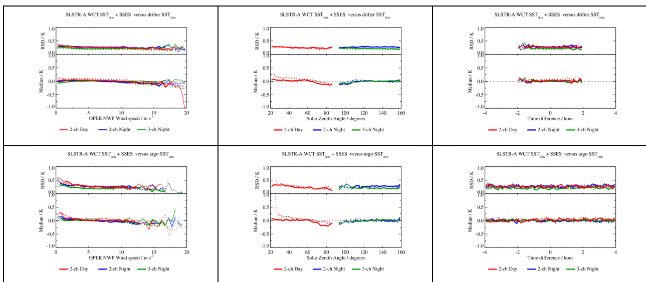
Figure 2: As per Figure 1 but with the addition of FK/C adjustments as described in the text.
