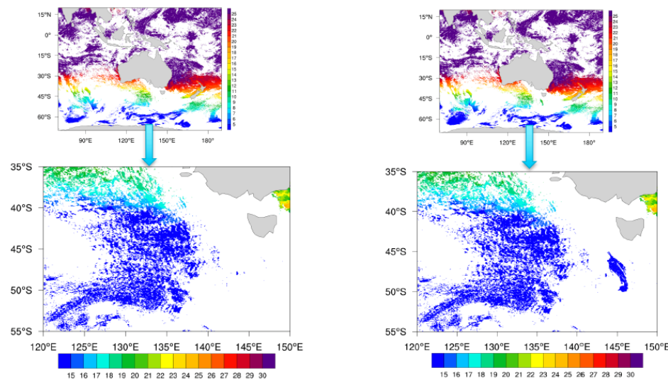
Figure 3: Sea surface temperatures with quality level 4 and 5 for L3S-1day night file from (a) NOAA-18, Metop-B, NPP and N20 and (b) NOAA-18, Metop-B, NPP, N20, Sentinel-3A and Sentinel-3B for 31 January 2020.
