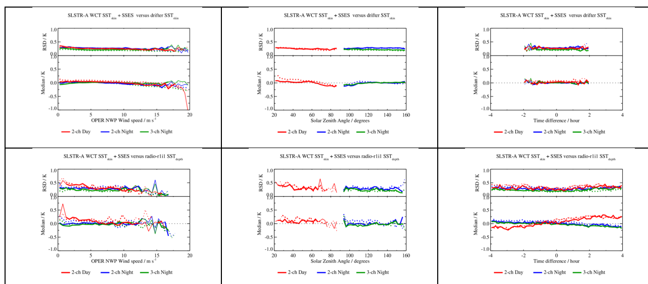
Figure 3: As per Figure 2 but comparing drifters (upper) and ship-borne radiometers.
