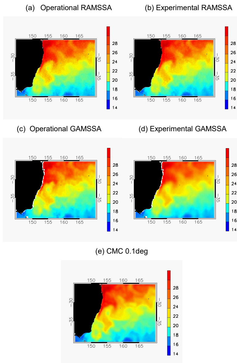
Figure 3: Example of foundation SST in the East Australian Current for 1 st April 2020 from daily Multi-sensor L4 analyses (a) operational RAMSSA, (b) experimental RAMSSA (ingesting VIIRS L3U SST), (c) operational GAMSSA, (d) experimental GAMSSA (ingesting VIIRS L3U SST) and (e) CMC0.1deg (ingesting VIIRS L3U SST) (Brasnett and Surcel Colan, 2016).
