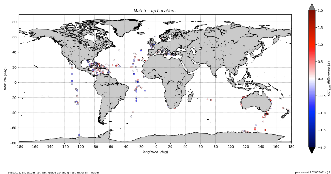
Figure 6: SLSTR Match-up locations for ships4sst data, 2016 to 2018.
