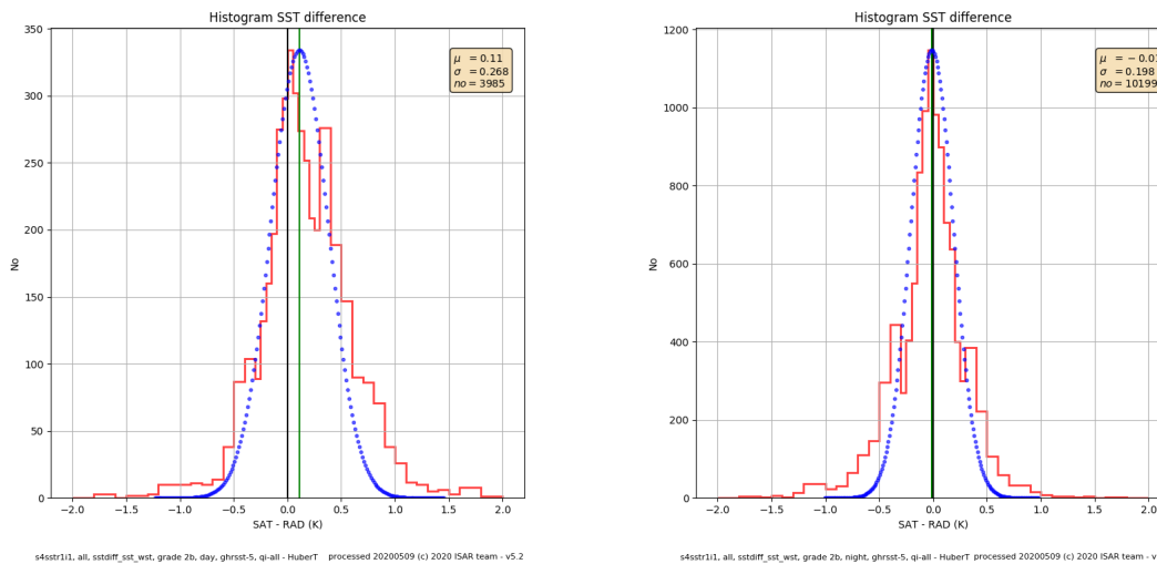
Figure 7: Histograms for the SLSTR Validation results, 2016 to 2018. The left plot shows the histograms for daytime matches and the right hand plot for nighttime matches for the WST product, GHRSSST quality level 5 and match-up grade 2b.
