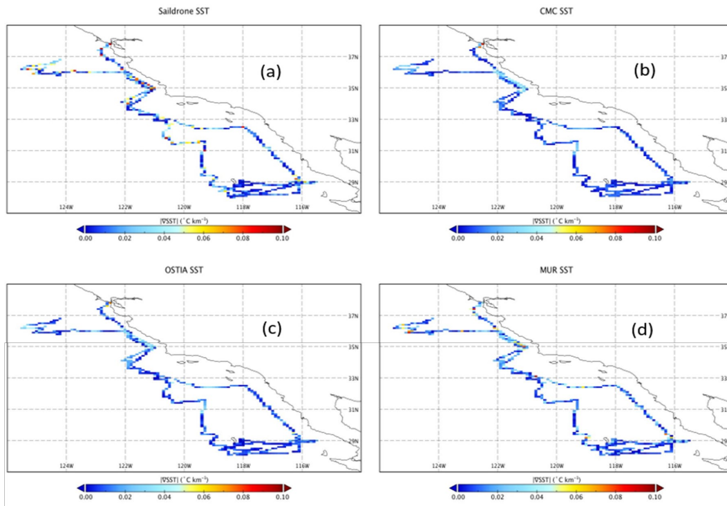
Figure 1: SST gradients
