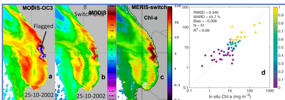
Figure 2: MODIS OC3 Chl-a (a), MODIS switch Chl-a (b) and MERIS switch Chl-a for 25 October 2002 in the SBUS (31°-34° S; 17°-19° E). The colour bars adjacent to the maps represent Chl-a in \text{mg m}^{-3} . Scatterplot showing the relationship between in situ Chl-a and satellite-derived reflectance from MERIS (circles) and OLCI (triangles) (Smith et al. 2018). The colour bar indicates the weighting of the G2B algorithm.
