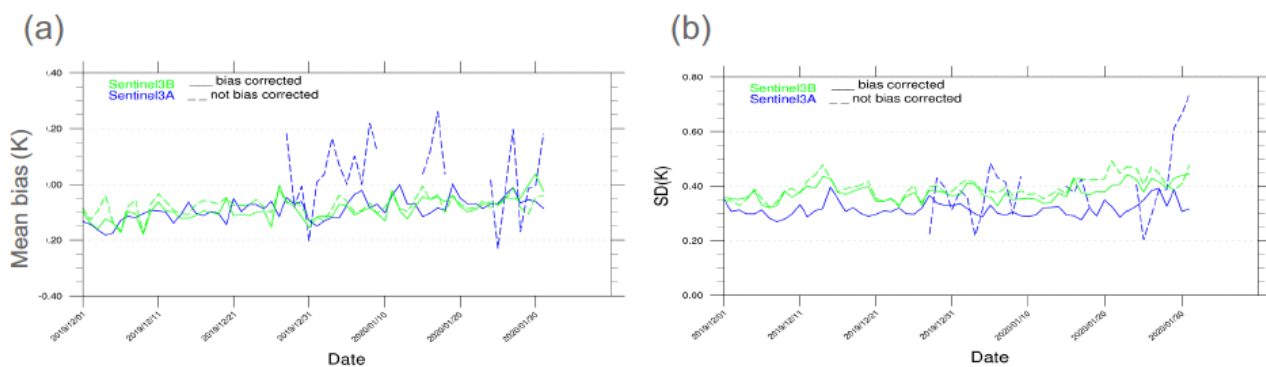
Figure 5: L3S-1day, night only, daily statistics, 1 Dec 2019 - 31 Jan 2020, QL ≥ 4, (a) Mean bias and (b) standard deviation when compared with SLSTR L3C SST. Note: Mean bias = SST - L3C SLSTR SST. Matchup thresholds: < 10 km distance and < 6 hr time.
