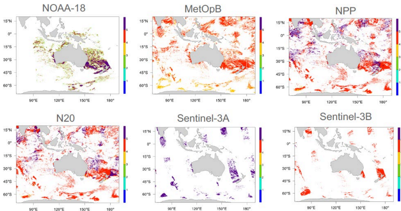
Figure 1: Remapped quality level for L3C-1day night file for 31 January 2020.
